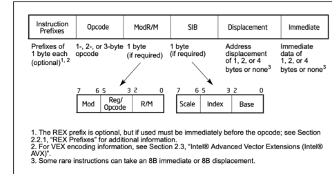
Figure 2-1. Intel 64 and IA-32 Architectures Instruction Format
